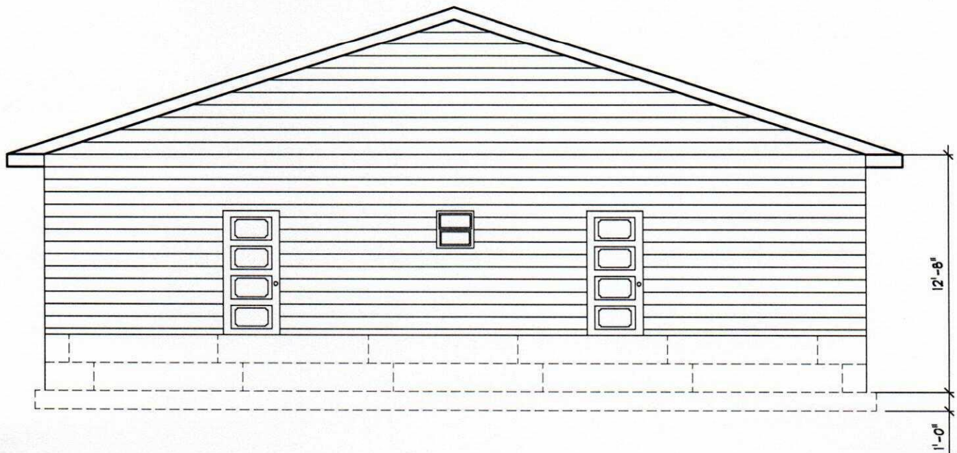
EAST VIEW
