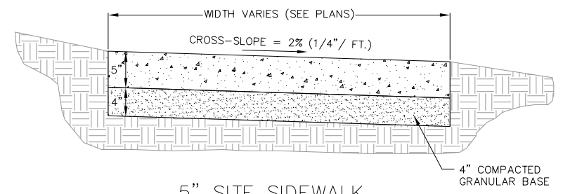
1 5" SITE SIDEWALK
