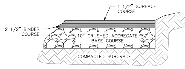
BITUMINOUS PAVEMENT DRIVES
