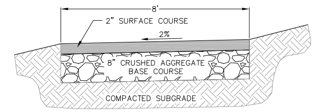
BITUMINOUS PAVEMENT BIKE PATH
