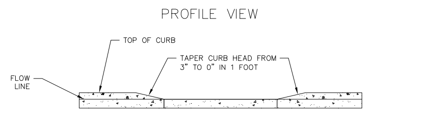
1 CURB CUT PROFILE VIEW
