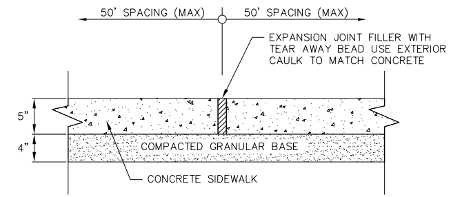
1 SIDEWALK EXPANSION JOINT
