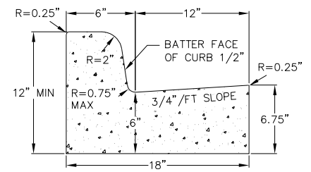
1 CURB AND GUTTER CROSS SECTION
