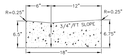
1 HANDICAP RAMP GUTTER CROSS SECTION
