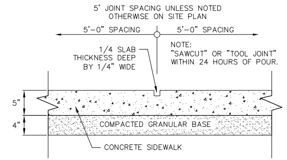
1 SIDEWALK CONTROL JOINT
