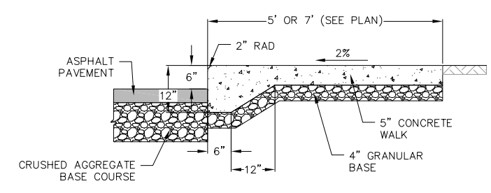
1 CURBED SIDEWALK SITE DETAIL 1 NOT TO SCALE
