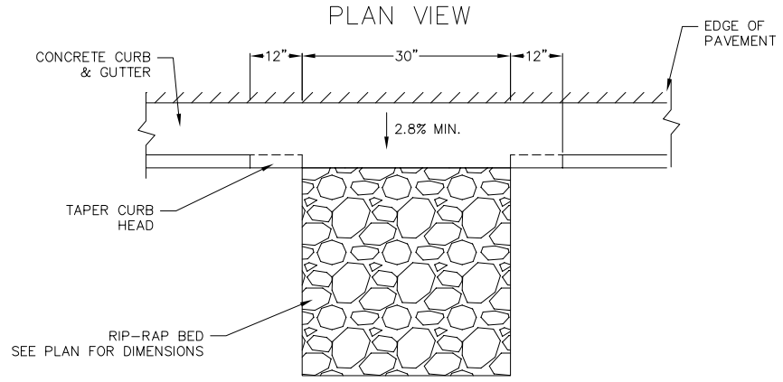
1 CURB CUT PLAN VIEW
