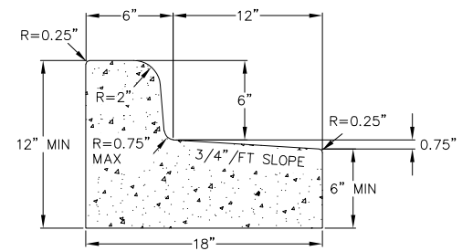
1 CURB AND GUTTER REJECT SECTION
