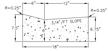
1 DRIVEWAY GUTTER CROSS SECTION
